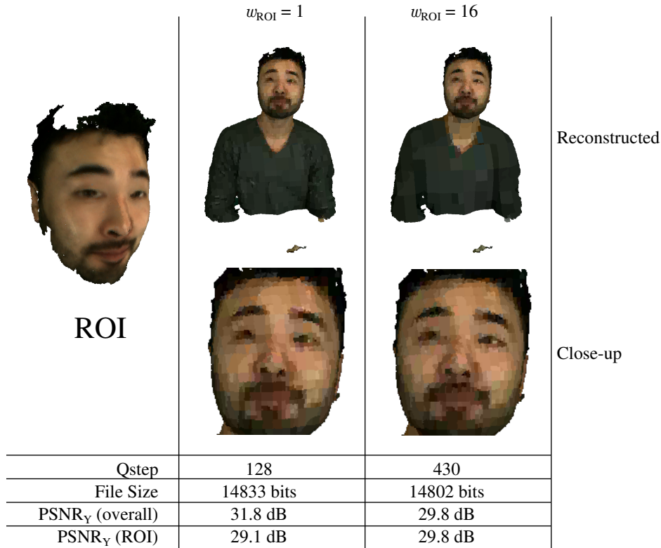
Figure 6.14: A frame of the point cloud David encoded with w_{ROI} equals to 1 and 16. The quantization step size was adjusted to yield similar encoded file sizes. A close-up of the reconstructed point cloud is also shown.
