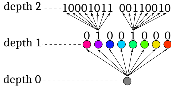
Figure 2.7: Octree signaling. Once a node is divided into 8 nodes, one byte is used to signalize which nodes are occupied. At depth = 1 , only two nodes are occupied: the second and the fifth, signaled by the byte 01001000. Only the occupied nodes are further divided and we send one byte for each occupied node at depth = 2 . In this example, assuming depth = 2 is the last division of this geometry, the sequence 010010001000101100110010 is enough to encode the position of the 7 voxels in this tiny point.
