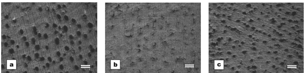
FIGURE 4: Photomicrography of transversal section of hardwood attacked by Gloeophyllum trabeum . a: Couratari oblongifolia ; b: Couratari guianensis and c: Couratari stellata . Scale bars = 1000 \mu m.
