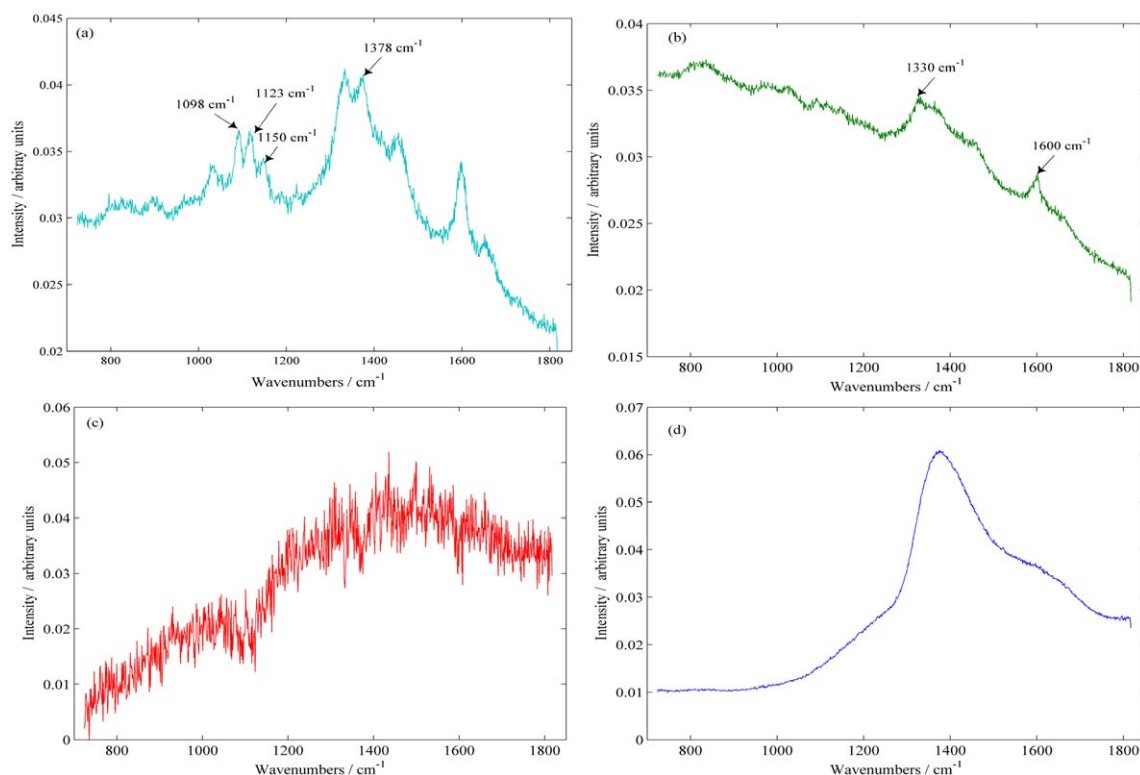
Figure 5. MCR-ALS recovered Raman spectra for Eucalyptus: (a) cellulose; (b) lignin; (c) background and (d) glass slide.
