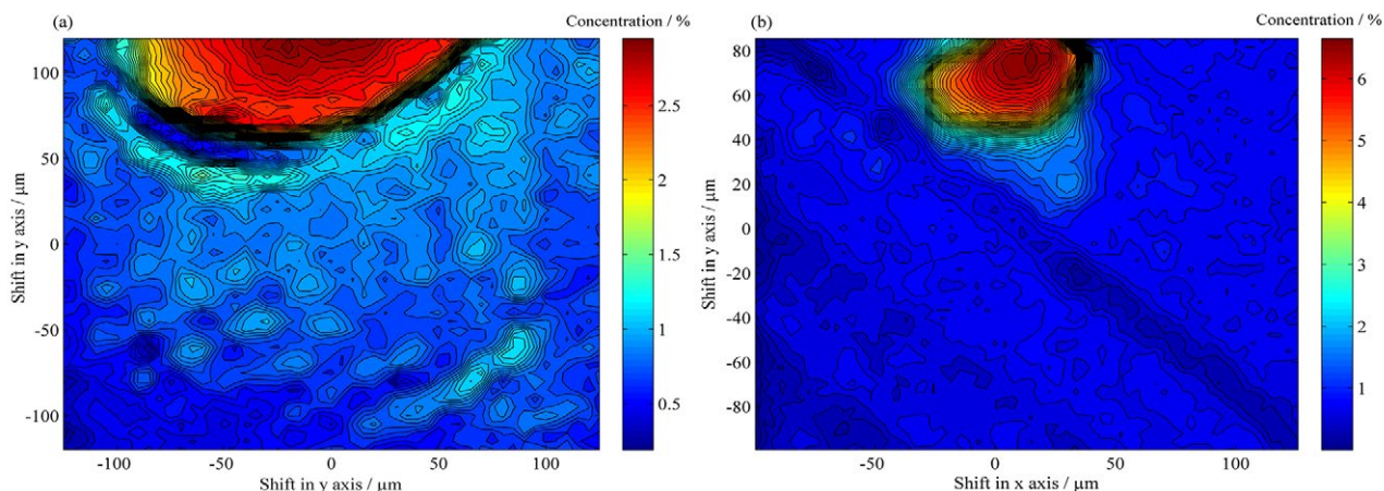
Figure 6. Intensity map related to the glass slide (a) Mahogany; (b) Eucalyptus.
