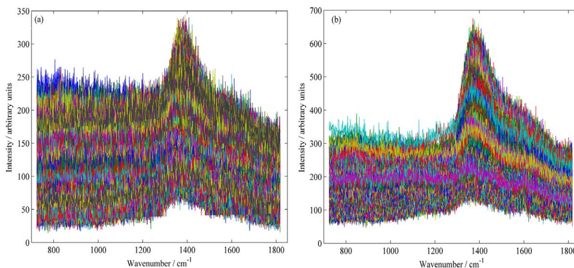
Figure 3. Raw data spectra: (a) Mahogany; (b) Eucalyptus.
