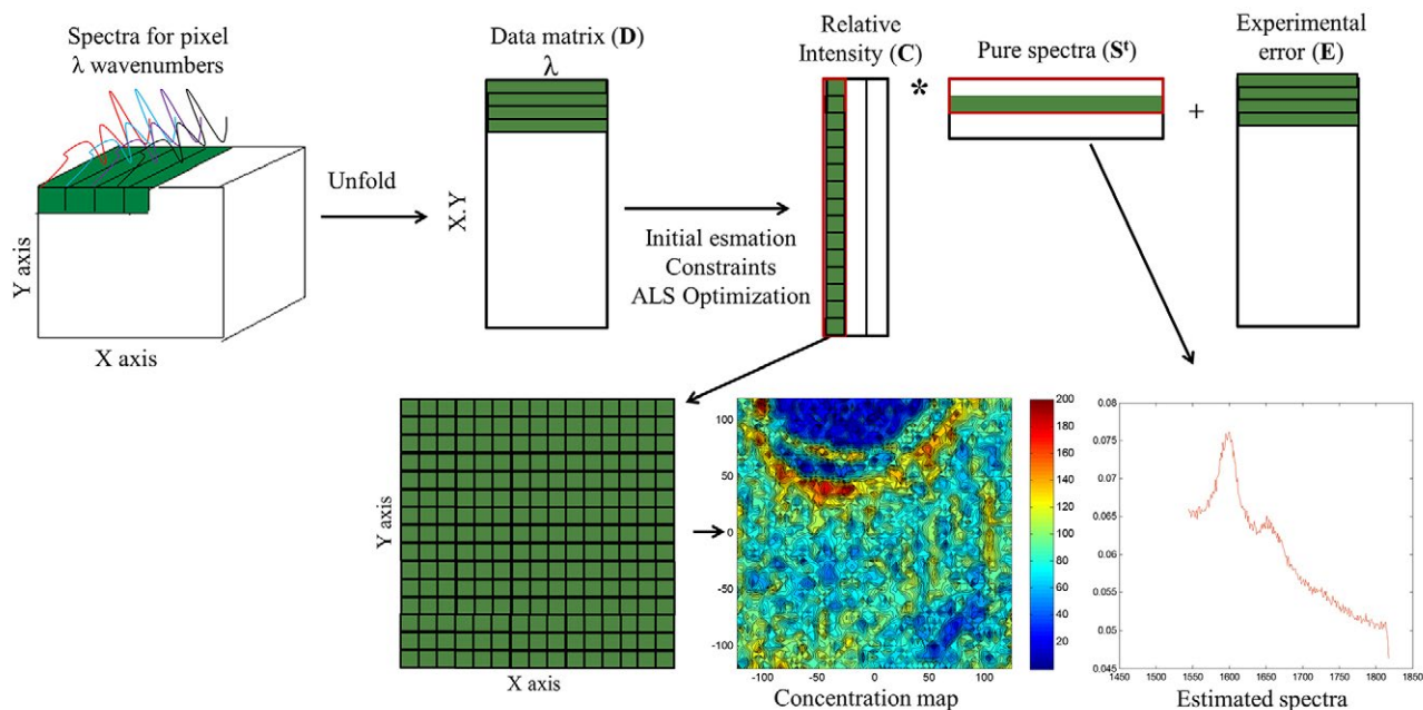
Figure 2. Schematic representation of bilinear matrix decomposition of a hyperspectral image using the MCR-ALS method.
