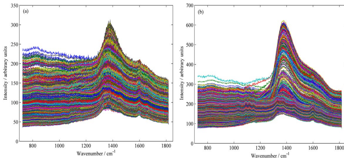
Figure 4. Data matrix spectra after filter based on principal component analysis for: (a) Mahogany; (b) Eucalyptus.
