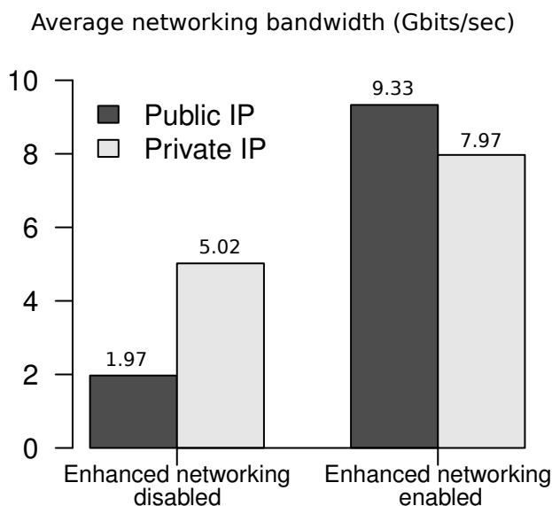
Figure 9.2 – Average network bandwidth of the Amazon EC2 instance c3.8xlarge when created with the default configuration; and using an internal (private) and an external (public) address for data transfer. The networking bandwidth was measured between two c3.8xlarge instances deployed in the region of Virginia (availability zone us-east-1a ) and running the iperf [168] application during one hour for each configuration scenario
