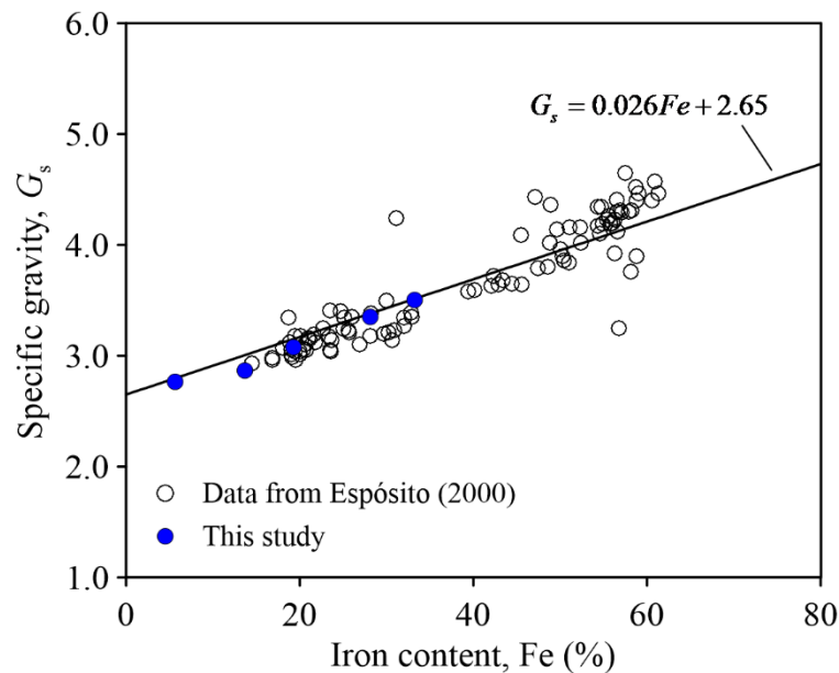
Figure 3.5. Relationship between specific gravity and iron content
