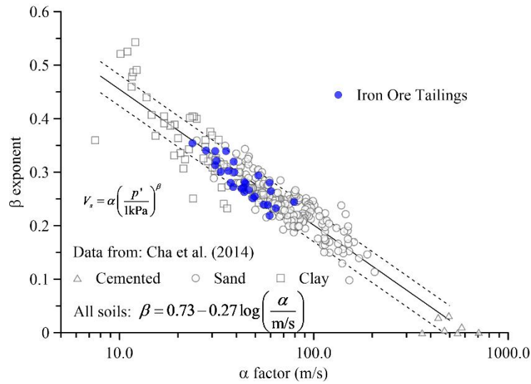
Figure 4.22. Inverse relationship between the \beta -exponent and the \alpha -factor. The cemented, sand and clay data were obtained from Cha et al. (2014).
