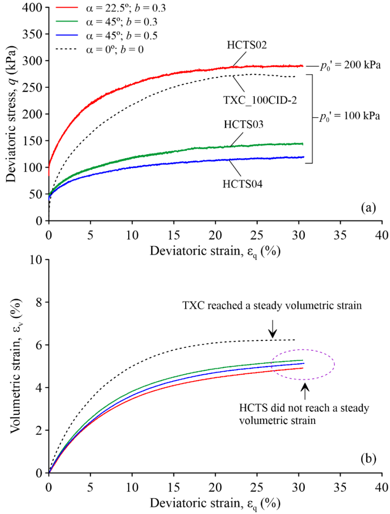
Figure 4.8. Stress–strain behaviour drained tests: (a) q - \epsilon_q plot; (b) \epsilon_v - \epsilon_q plot.
