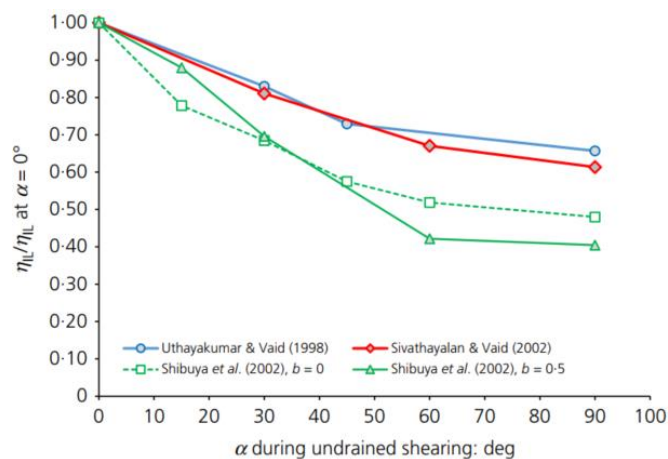
Figure 2.7. Effect of principal stress direction on instability stress ratio (Reid, 2020).
