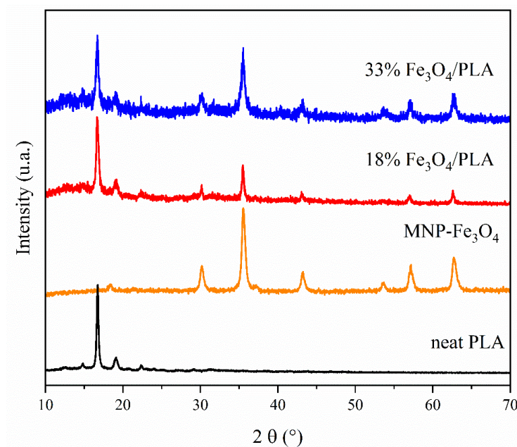
Figure 11. XRD patterns of the samples: pure PLA, MNP- \text{Fe}_3\text{O}_4 , and MNP- \text{Fe}_3\text{O}_4/\text{PLA} composites with 18% and 33% loadings.
