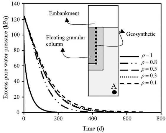
Fig. 14. Dissipation of excess pore water pressure for floating columns.
