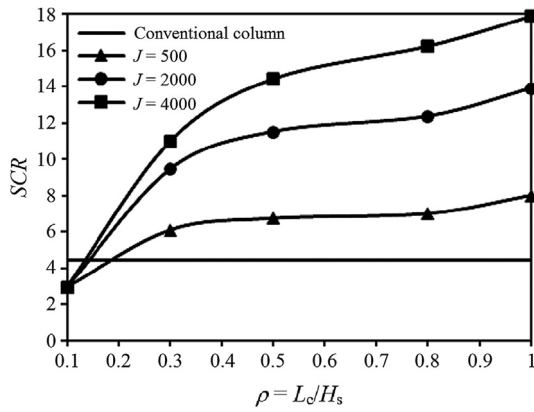
Fig. 15. Stress concentration factor versus floating ratio.
