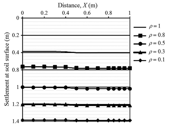
Fig. 10. Settlement at the soil surface for different floating ratios ( \rho ).
